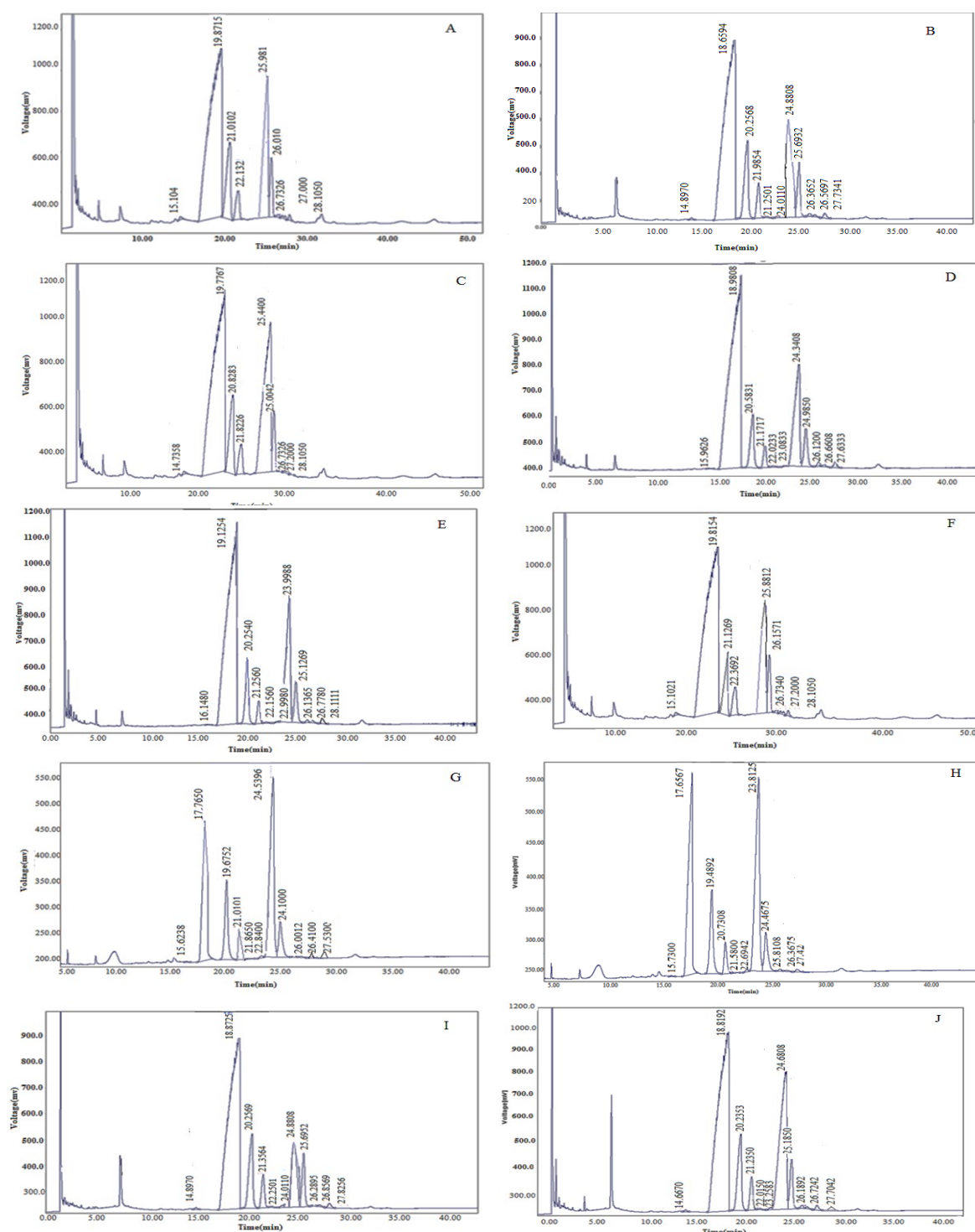
Figure 1: GC Chromatograms of sterol fraction of sesame oil samples (A, B, C, F, G, H, I, J: oils extracted with cold-press; D and E: commercially refined oils)
